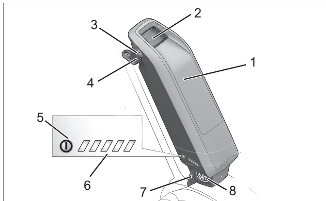
Figure 13: Detailed drawing of the down tube or seat tube battery
