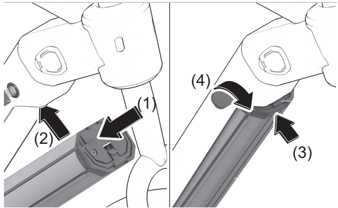
Inserting the integrated battery
