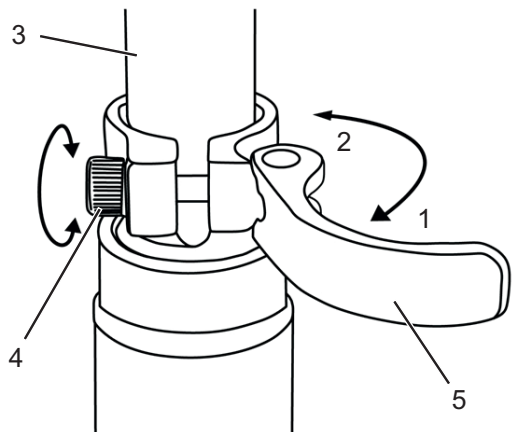
Figure 37: Seat post quick release (3) with clamping lever (5) and adjustment screw (4) in the open position (1) and in the direction of the closed position (2)
