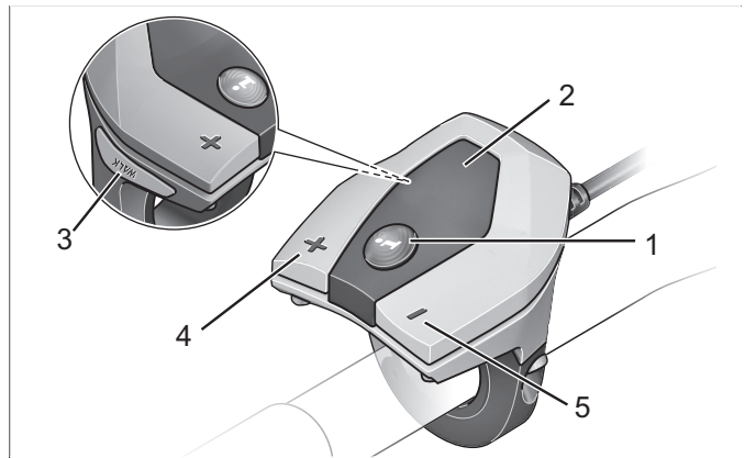
Overview of the control panel
