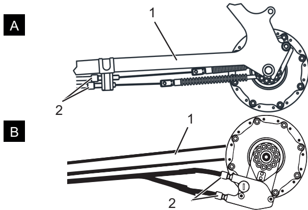
Figure 62: Adjusting sleeves (2) on two alternative versions (A and B) of a dual-cable cable-operated gear shift on the chain stay (1)
